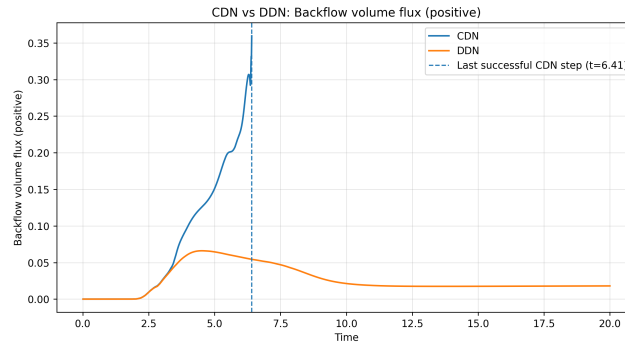
Figure 5: Backflow volume flux.
